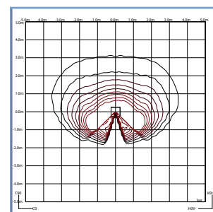
Courbes Isolux / Isolux curves
